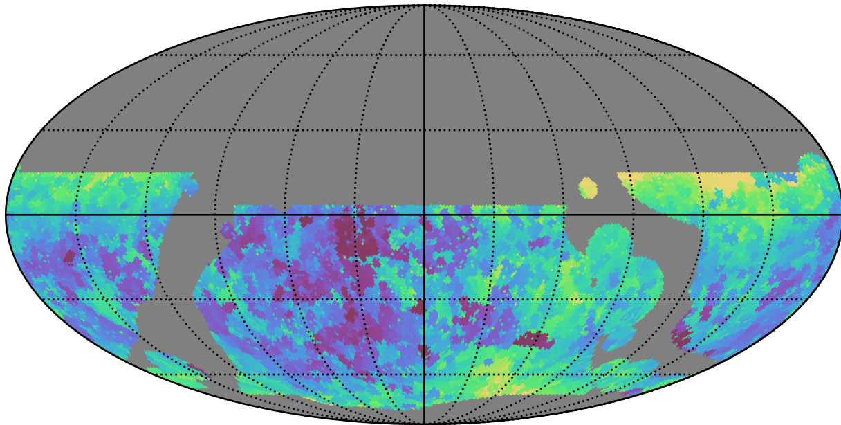
weather_cloudso0v3.5_10yrs WFD r band: Min seeingEff
