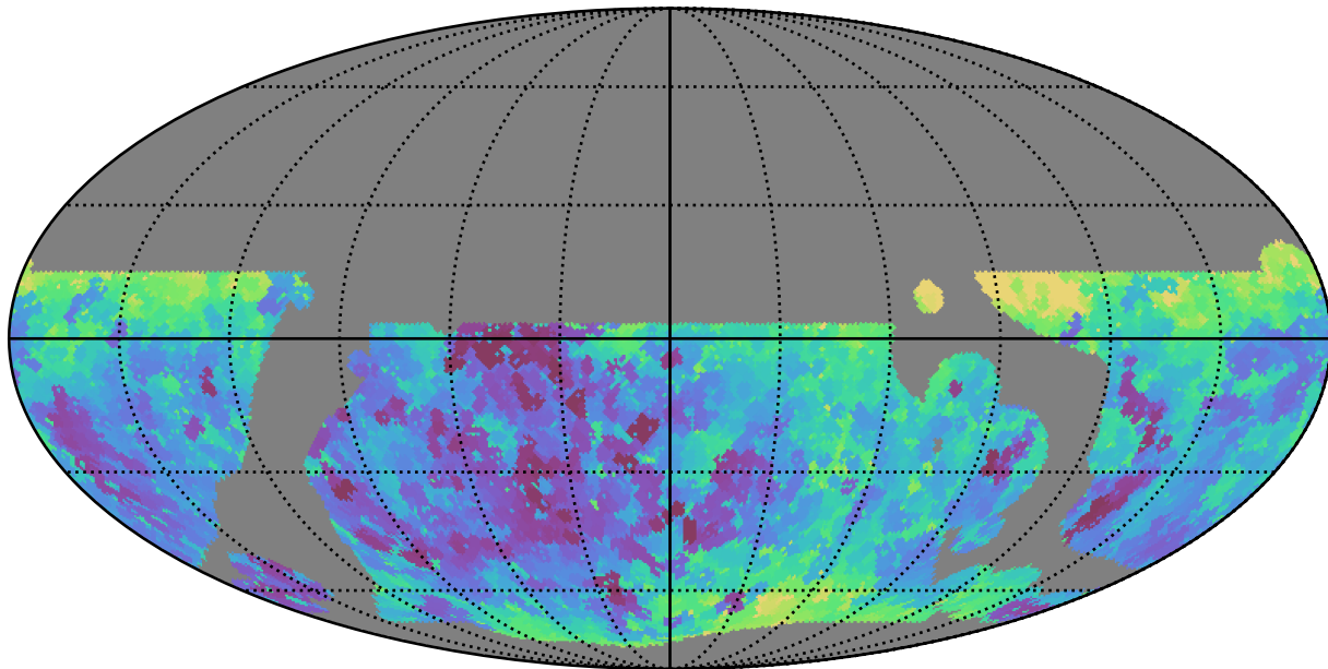
weather_cloudso0v3.5_10yrs WFD i band: Min seeingEff
