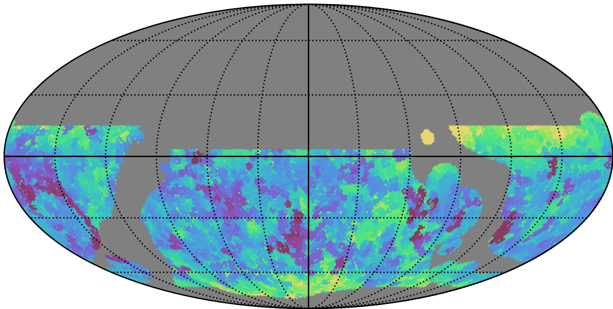
weather_cloudso0v3.5_10yrs WFD g band: Min seeingEff
