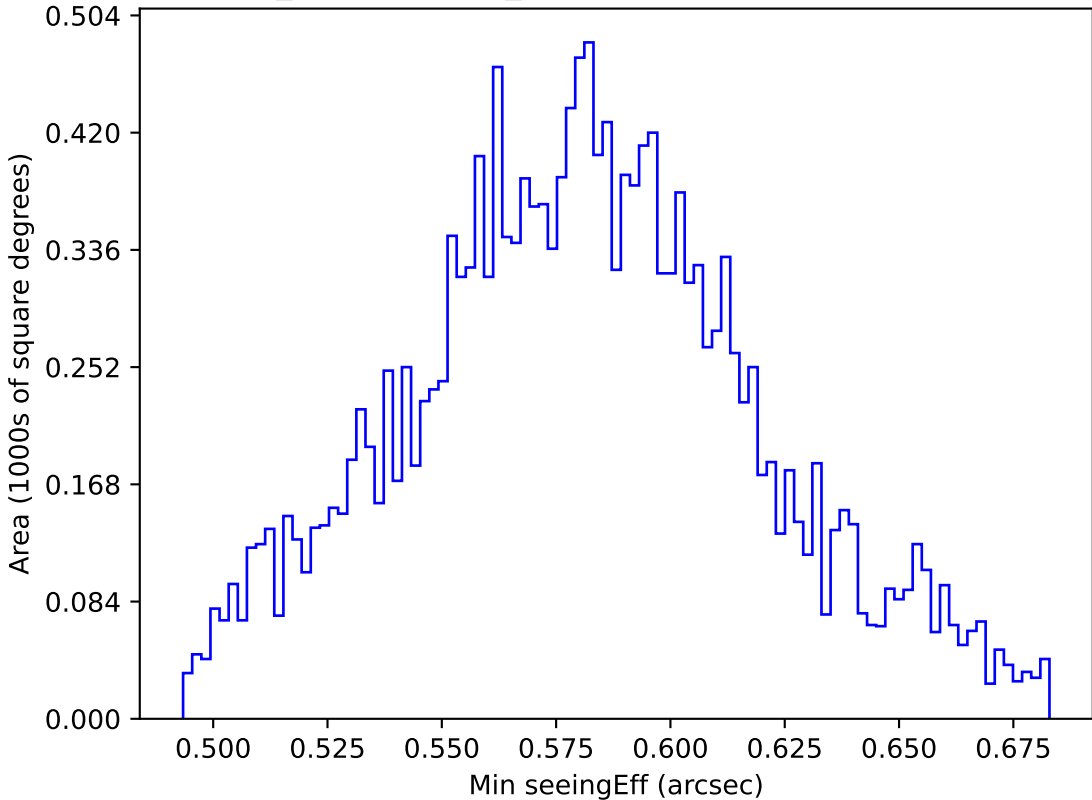
weather_cloudso0v3.5_10yrs WFD all bands: Min seeingEff
