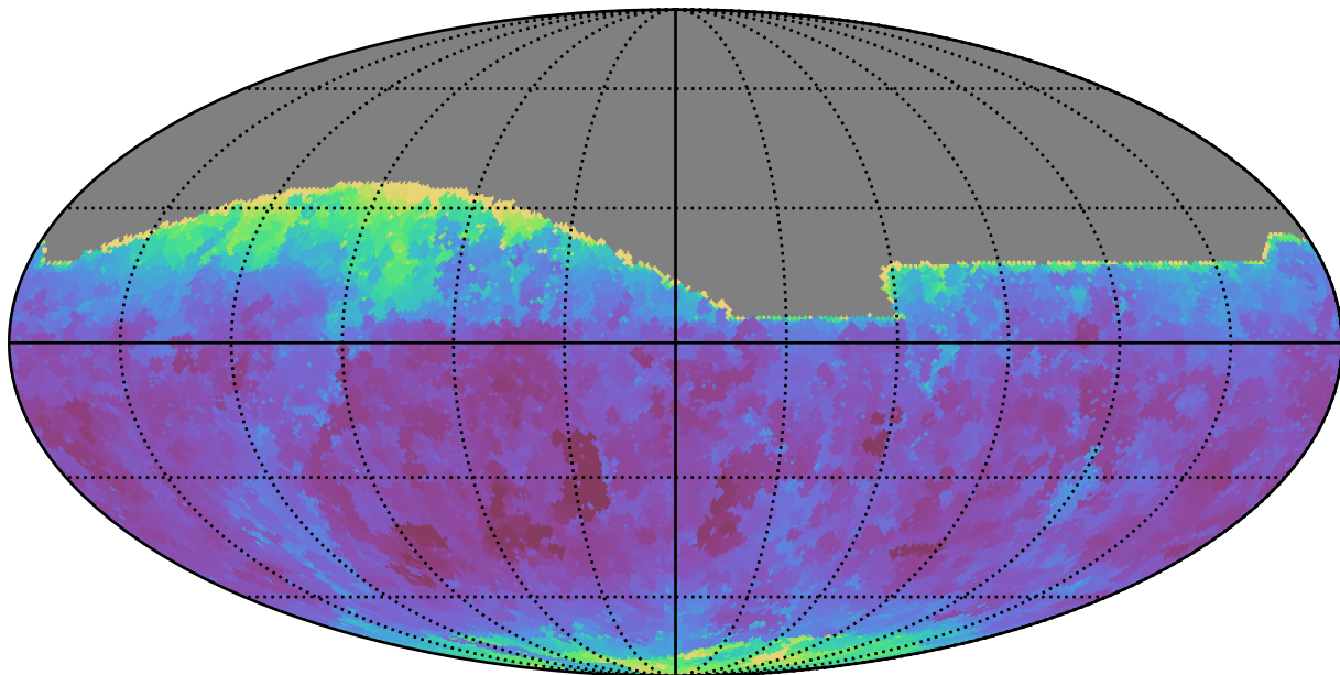
weather_cloudso0v3.5_10yrs All sky z band: Min seeingEff
