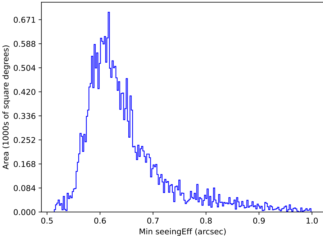
weather_cloudso0v3.5_10yrs All sky z band: Min seeingEff
