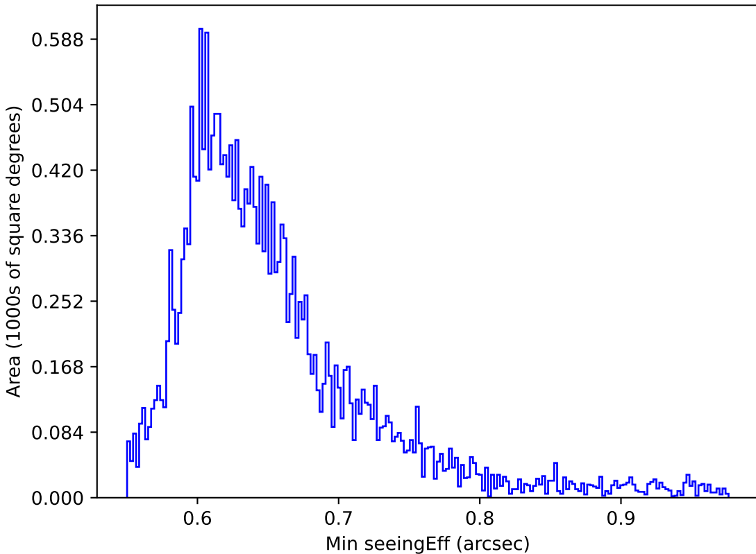
weather_cloudso0v3.5_10yrs All sky y band: Min seeingEff
