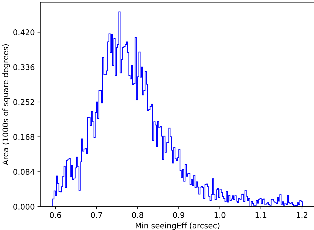
weather_cloudso0v3.5_10yrs All sky u band: Min seeingEff
