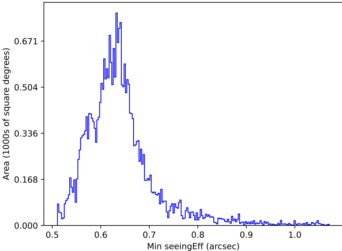
weather_cloudso0v3.5_10yrs All sky r band: Min seeingEff
