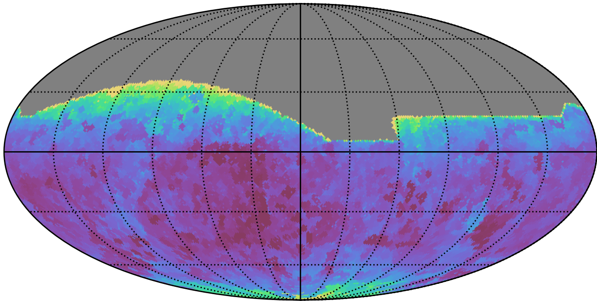
weather_cloudso0v3.5_10yrs All sky all bands: Min seeingEff
