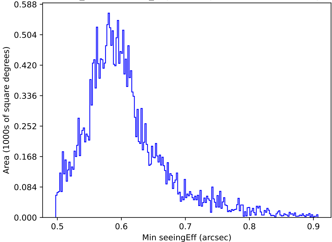
weather_cloudso0v3.5_10yrs All sky all bands: Min seeingEff
