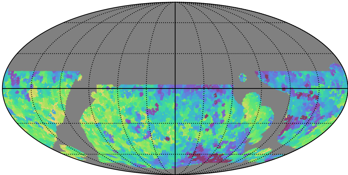
weather_cloudso0v3.5_10yrs WFD all bands: Min saturation_mag
