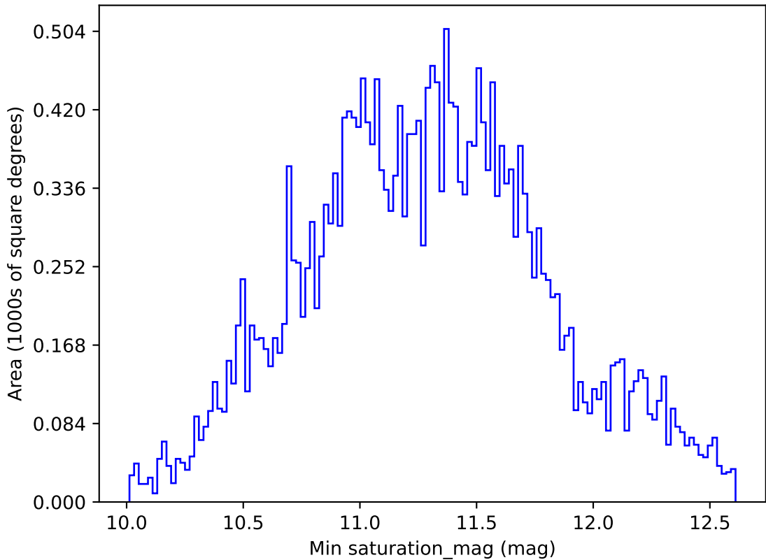
weather_cloudso0v3.5_10yrs All sky all bands: Min saturation_mag
