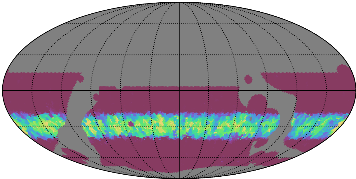
weather_cloudso0v3.5_10yrs WFD g band: Min normairmass
