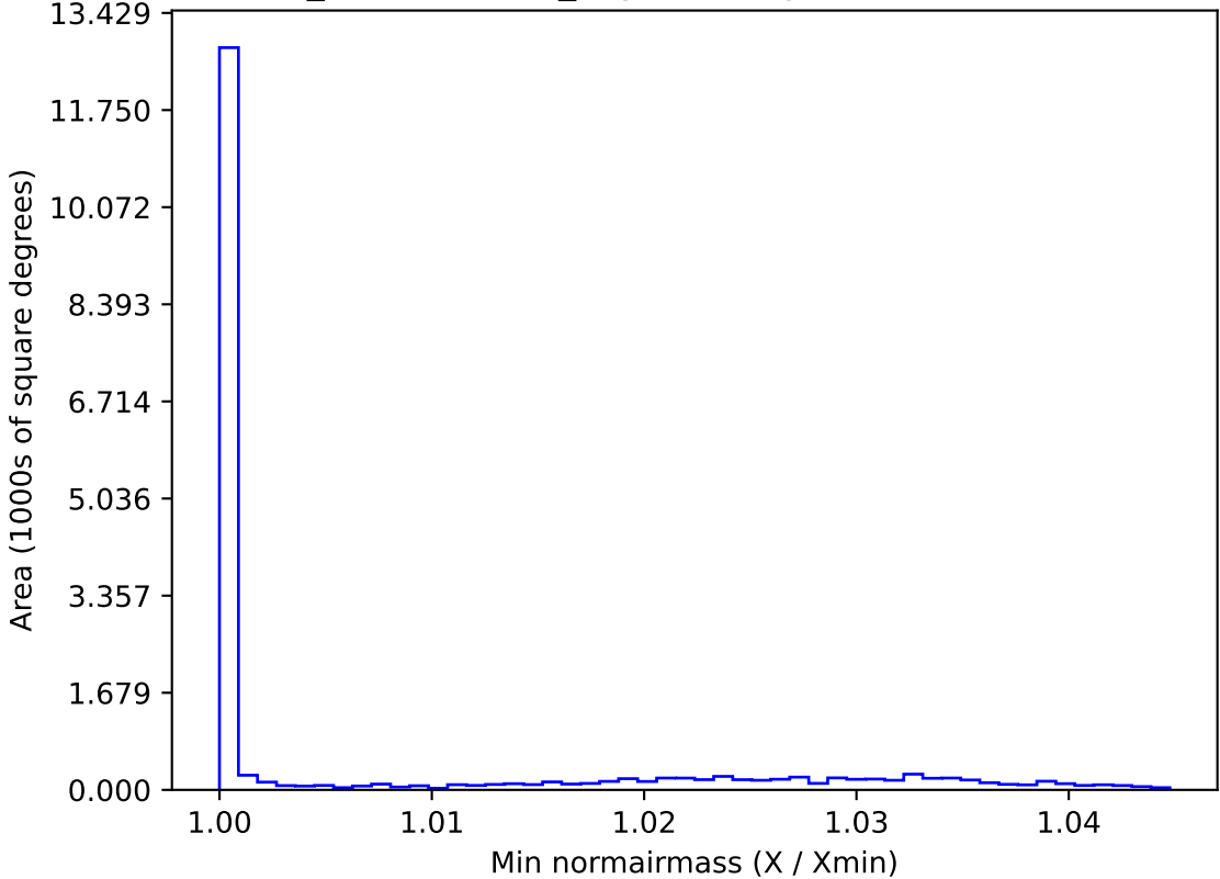
weather_cloudso0v3.5_10yrs WFD g band: Min normairmass
