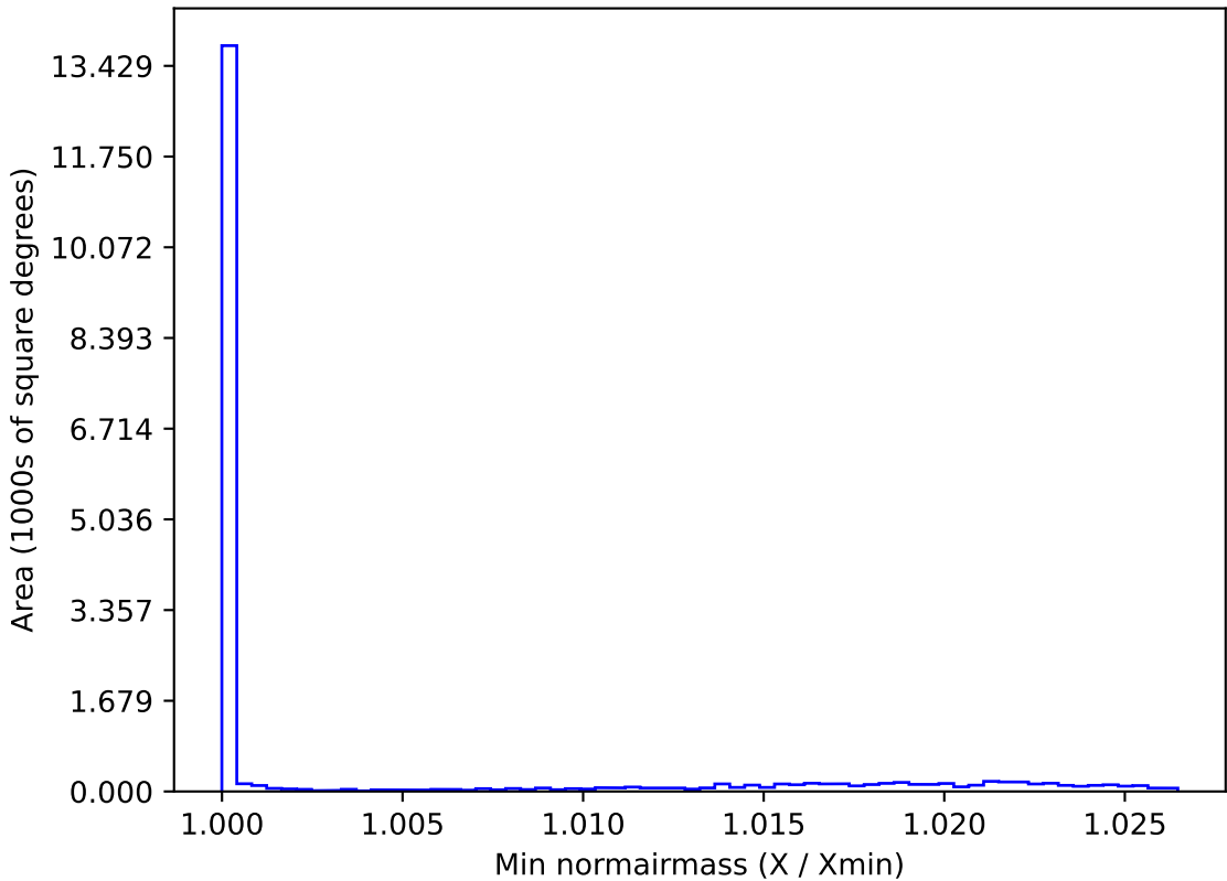
weather_cloudso0v3.5_10yrs WFD all bands: Min normairmass
