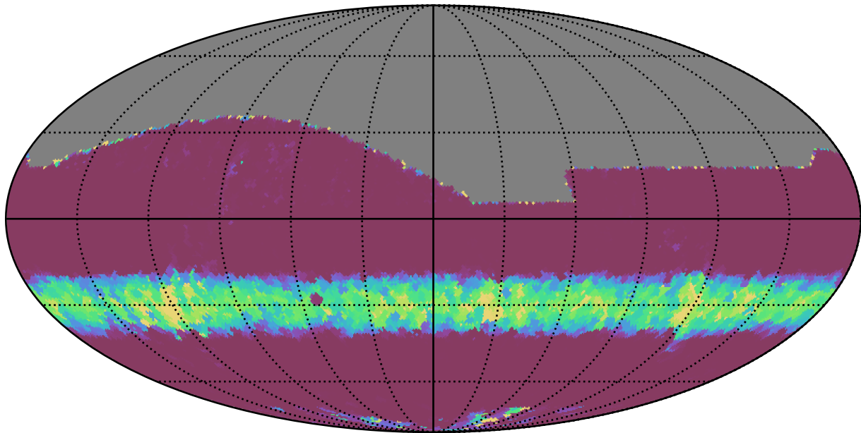
weather_cloudso0v3.5_10yrs All sky z band: Min normairmass
