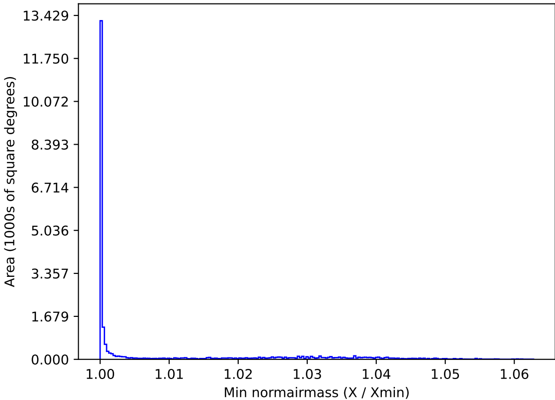
weather_cloudso0v3.5_10yrs All sky u band: Min normairmass
