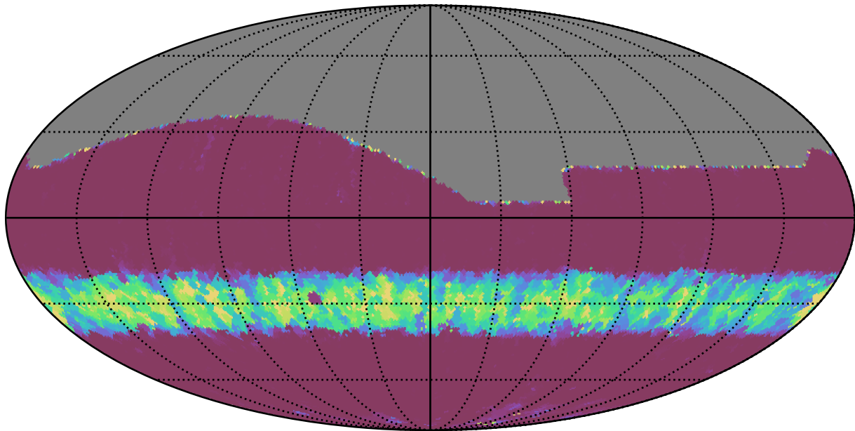
weather_cloudso0v3.5_10yrs All sky g band: Min normairmass
