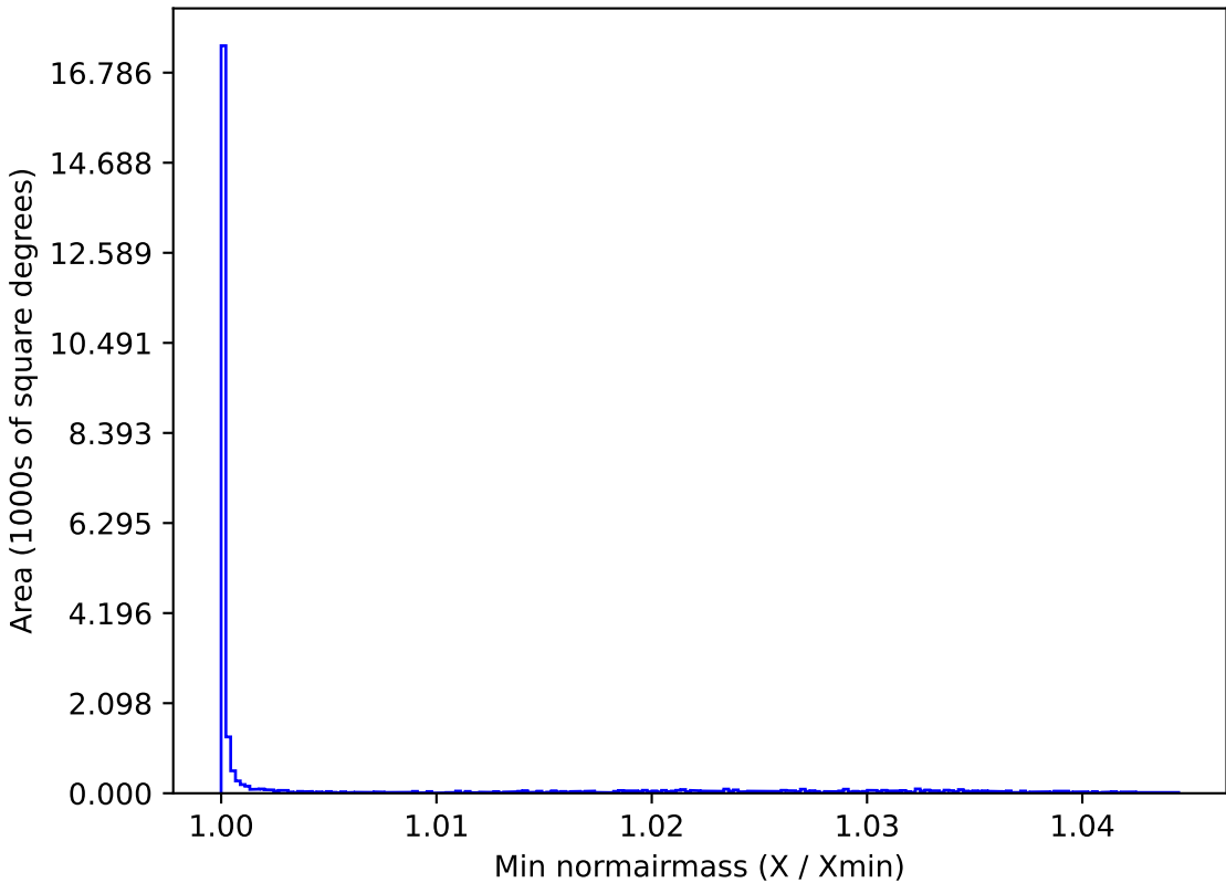
weather_cloudso0v3.5_10yrs All sky g band: Min normairmass
