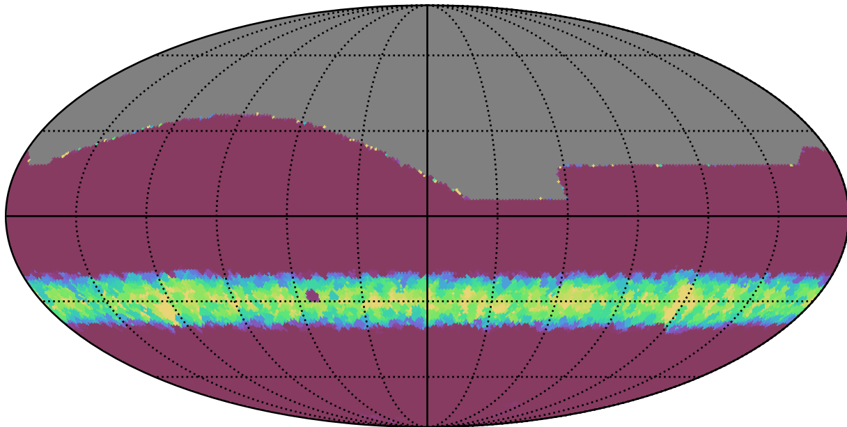
weather_cloudso0v3.5_10yrs All sky all bands: Min normairmass
