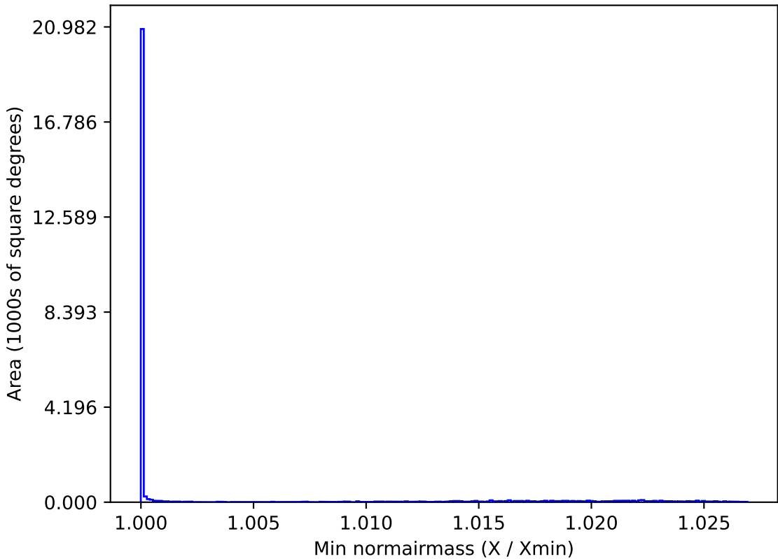
weather_cloudso0v3.5_10yrs All sky all bands: Min normairmass
