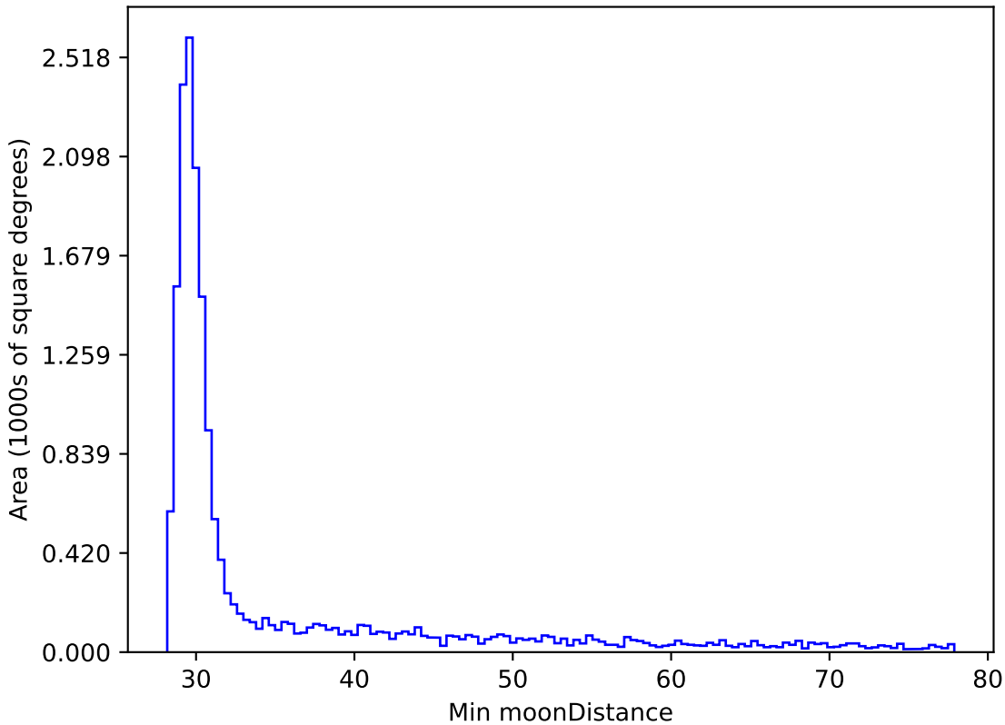
weather_cloudso0v3.5_10yrs WFD z band: Min moonDistance
