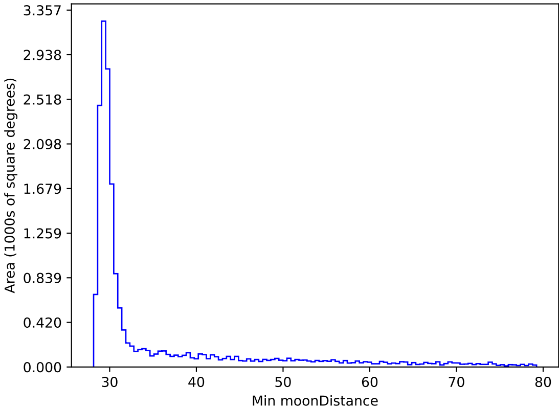
weather_cloudso0v3.5_10yrs WFD y band: Min moonDistance
