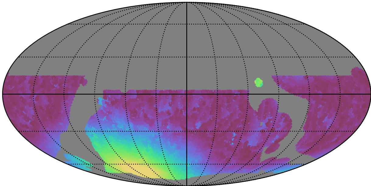
weather_cloudso0v3.5_10yrs WFD r band: Min moonDistance
