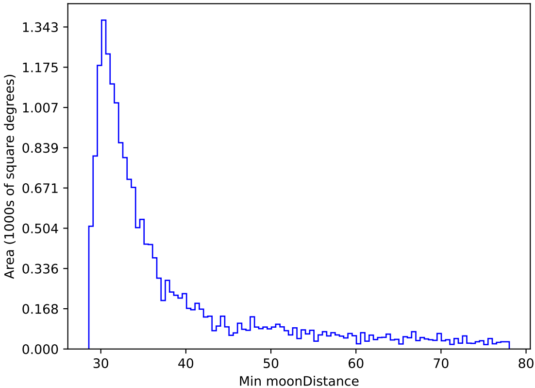
weather_cloudso0v3.5_10yrs WFD r band: Min moonDistance
