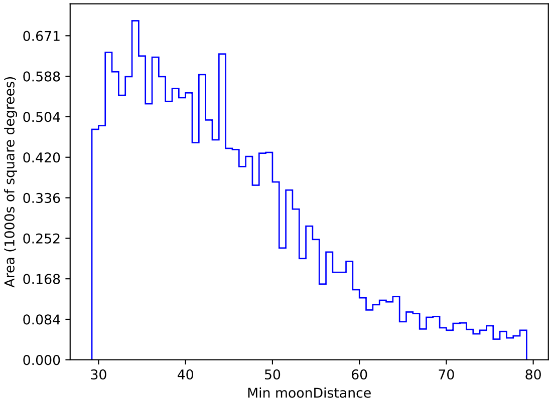
weather_cloudso0v3.5_10yrs WFD g band: Min moonDistance
