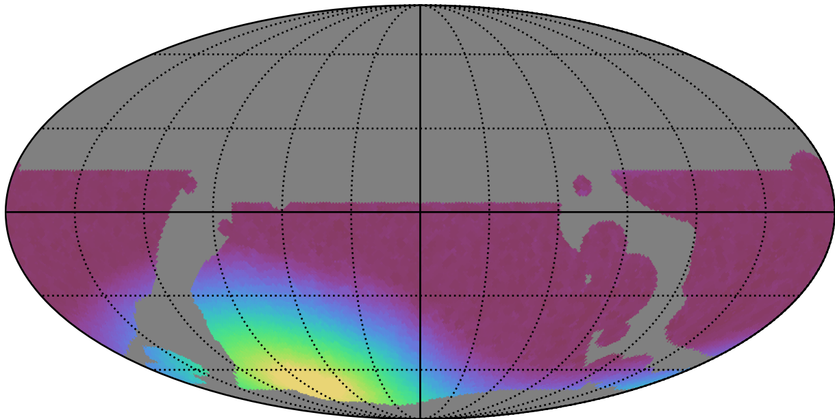
weather_cloudso0v3.5_10yrs WFD all bands: Min moonDistance
