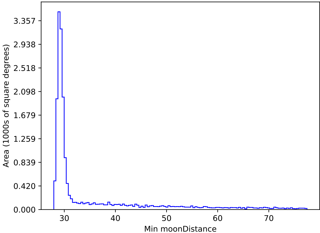
weather_cloudso0v3.5_10yrs WFD all bands: Min moonDistance
