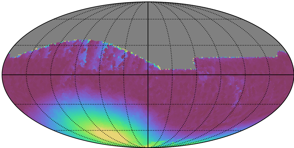
weather_cloudso0v3.5_10yrs All sky z band: Min moonDistance
