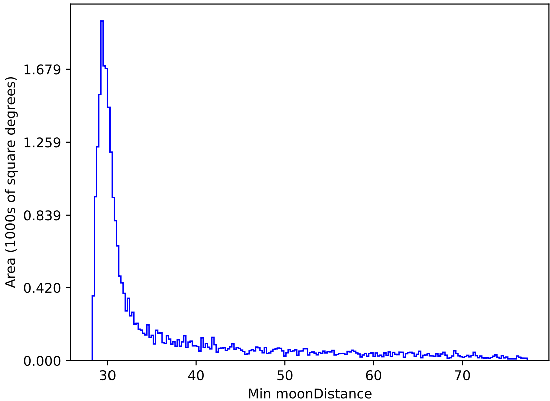
weather_cloudso0v3.5_10yrs All sky z band: Min moonDistance
