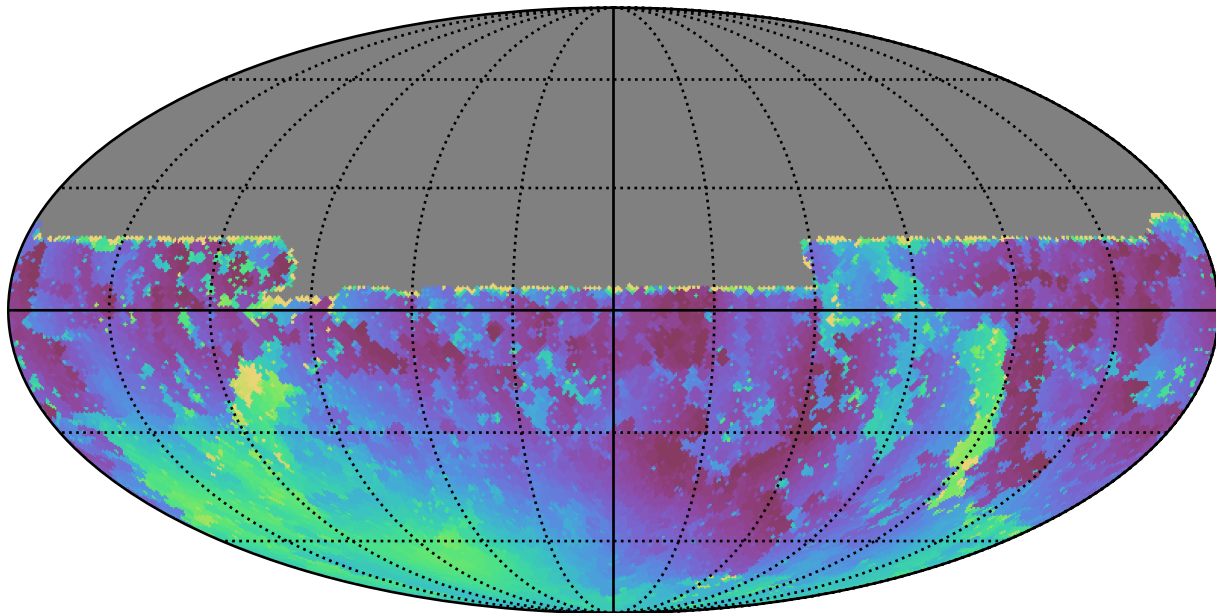
weather_cloudso0v3.5_10yrs All sky u band: Min moonDistance
