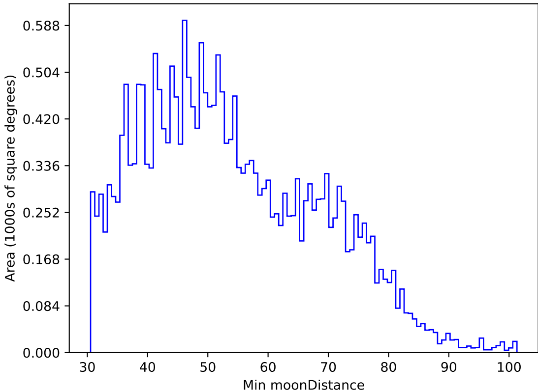
weather_cloudso0v3.5_10yrs All sky u band: Min moonDistance
