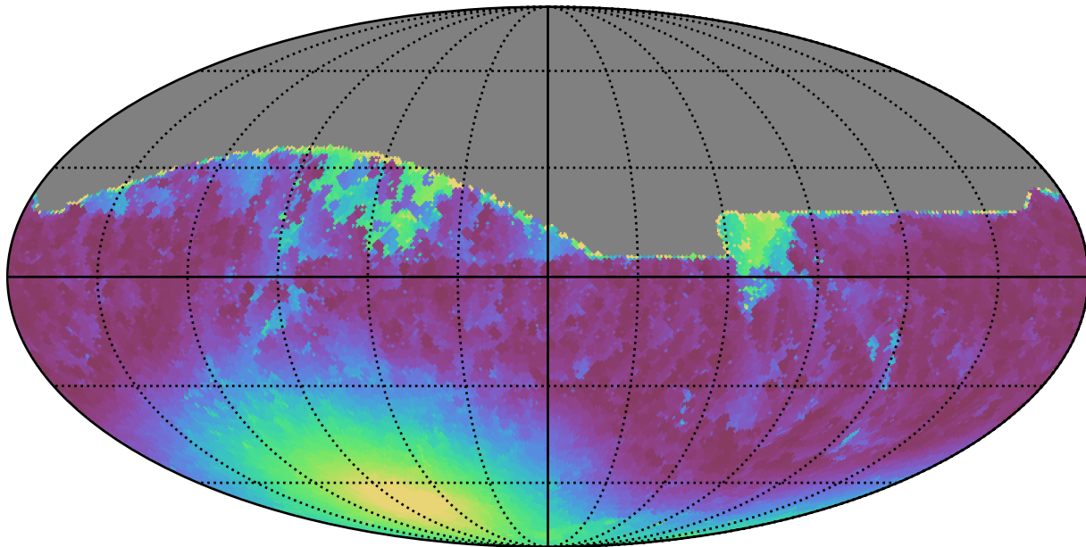
weather_cloudso0v3.5_10yrs All sky r band: Min moonDistance
