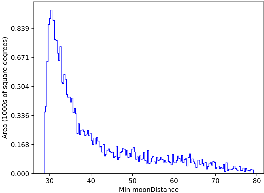
weather_cloudso0v3.5_10yrs All sky r band: Min moonDistance
