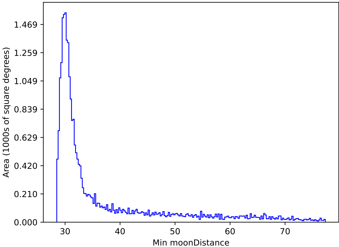
weather_cloudso0v3.5_10yrs All sky i band: Min moonDistance
