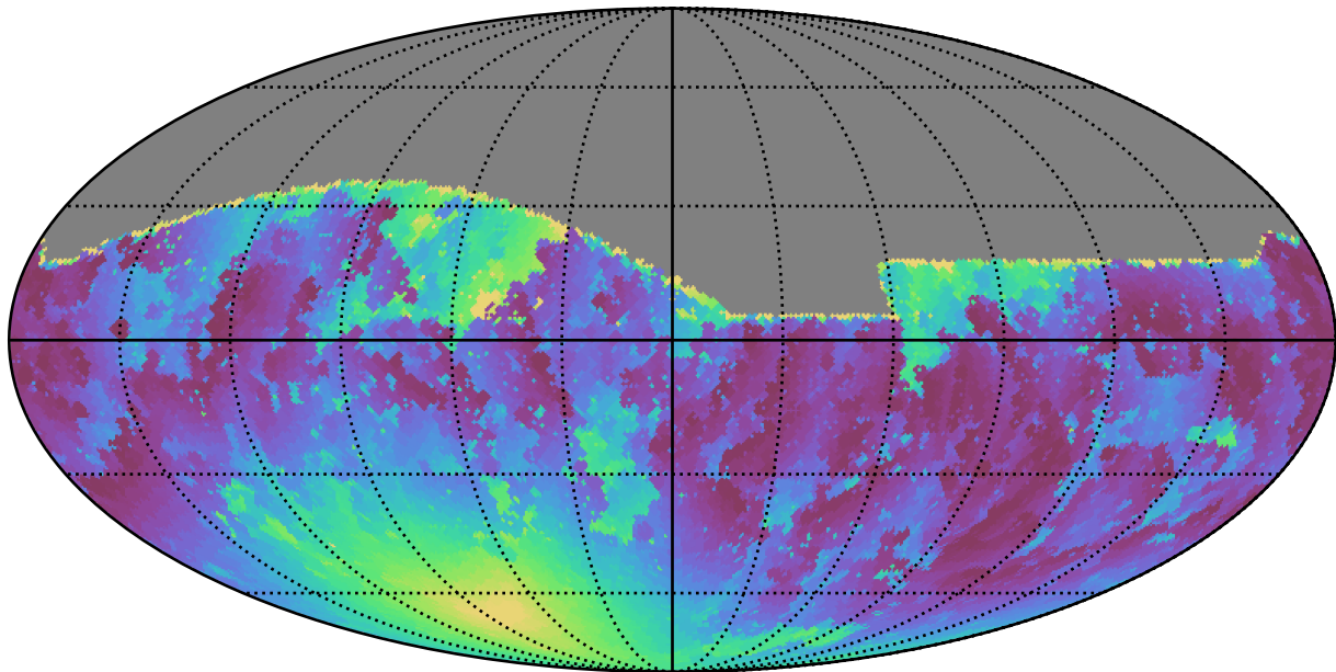
weather_cloudso0v3.5_10yrs All sky g band: Min moonDistance
