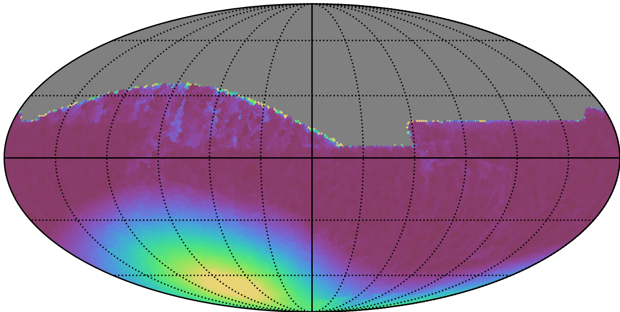
weather_cloudso0v3.5_10yrs All sky all bands: Min moonDistance
