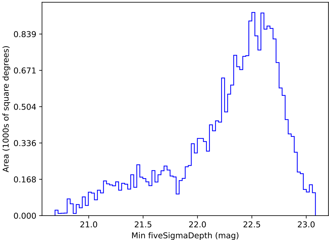
weather_cloudso0v3.5_10yrs Yr 1 z band: Min fiveSigmaDepth
