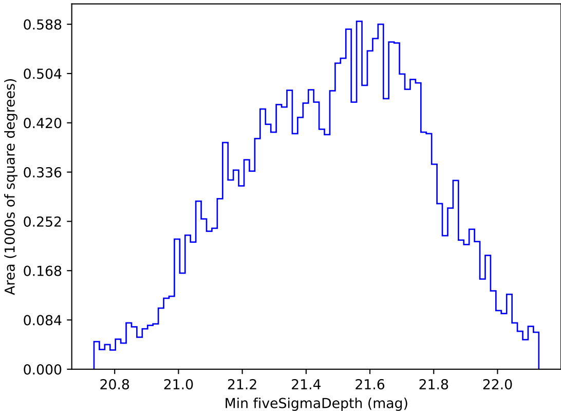
weather_cloudso0v3.5_10yrs Yr 1 y band: Min fiveSigmaDepth
