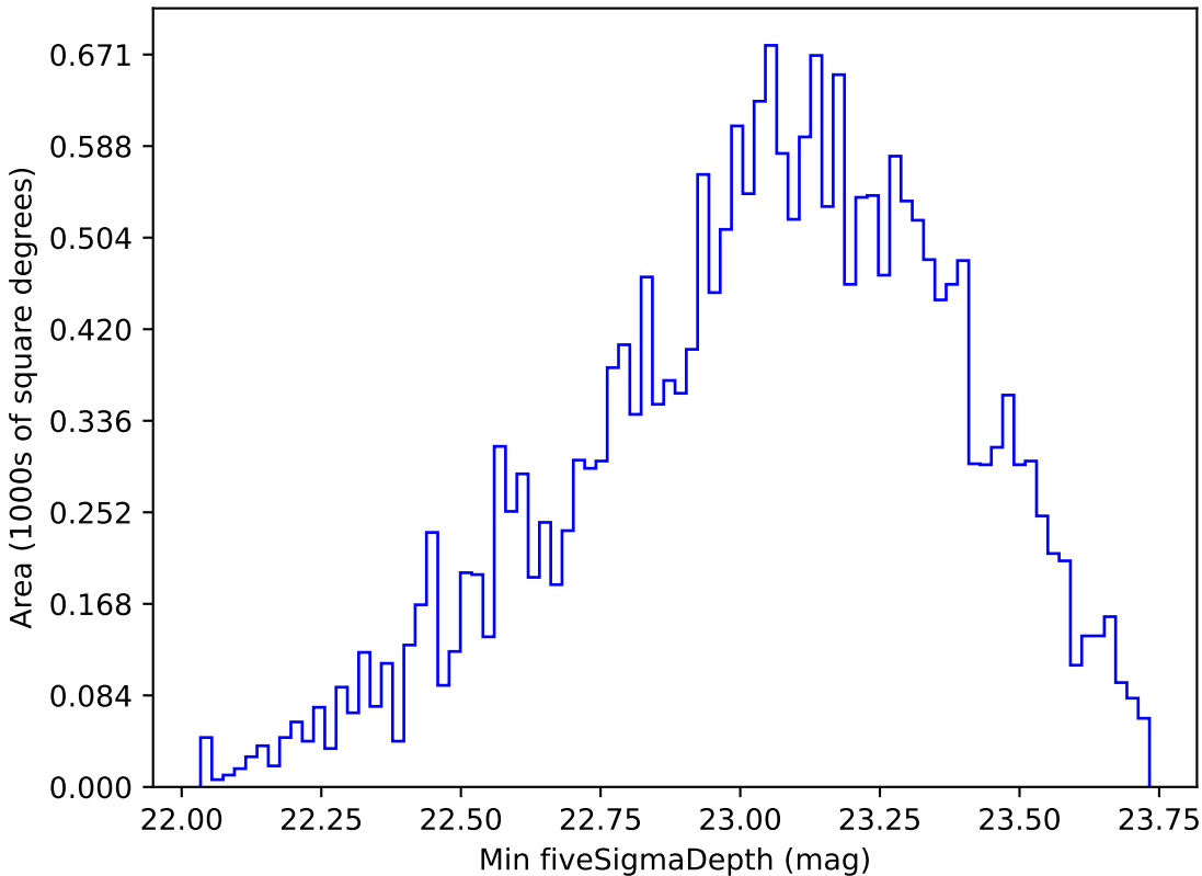
weather_cloudso0v3.5_10yrs Yr 1 u band: Min fiveSigmaDepth
