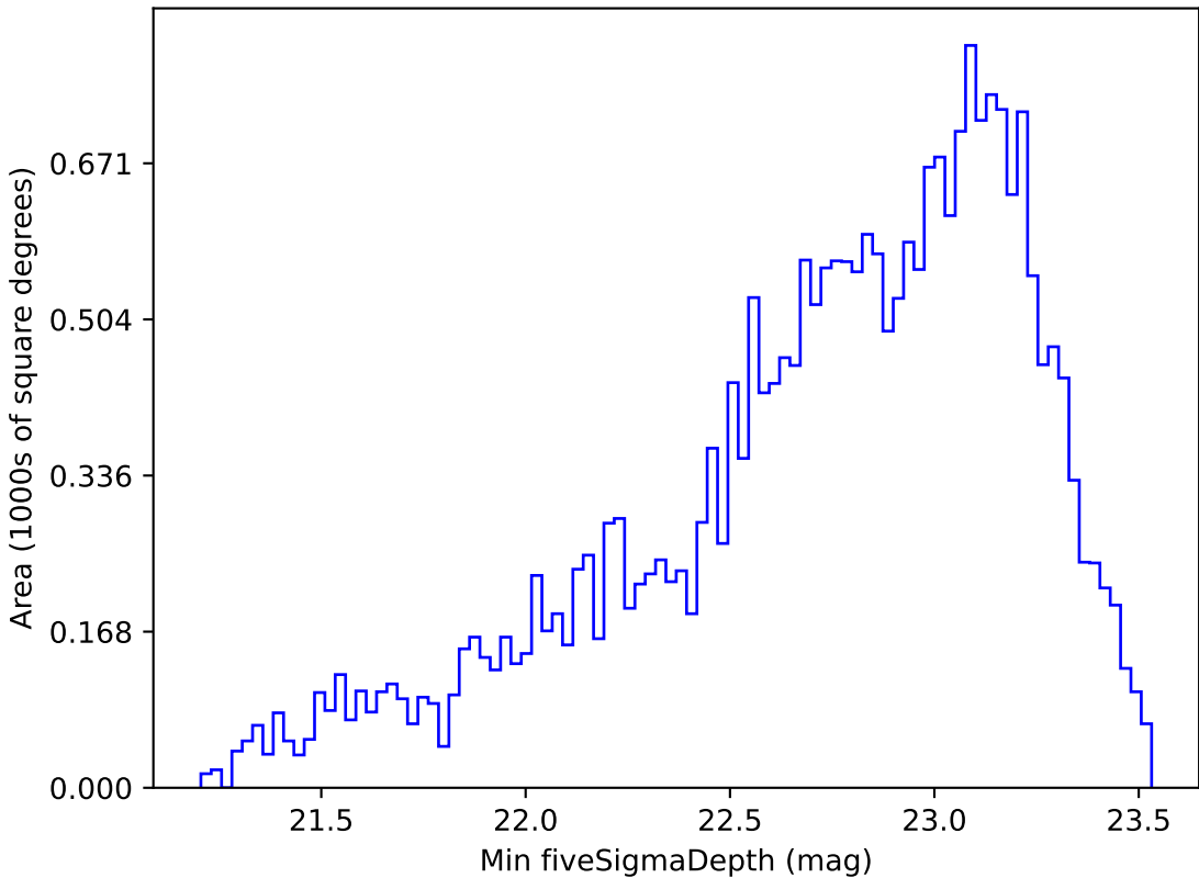
weather_cloudso0v3.5_10yrs Yr 1 i band: Min fiveSigmaDepth
