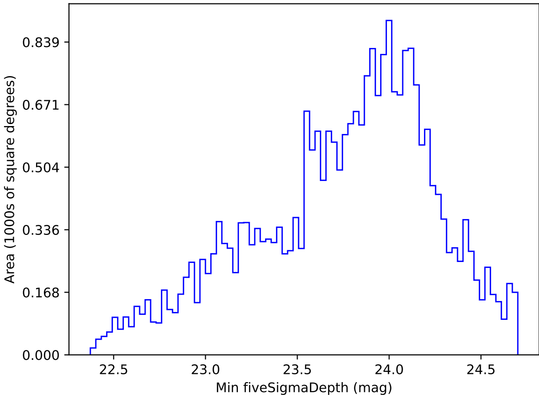
weather_cloudso0v3.5_10yrs Yr 1 g band: Min fiveSigmaDepth
