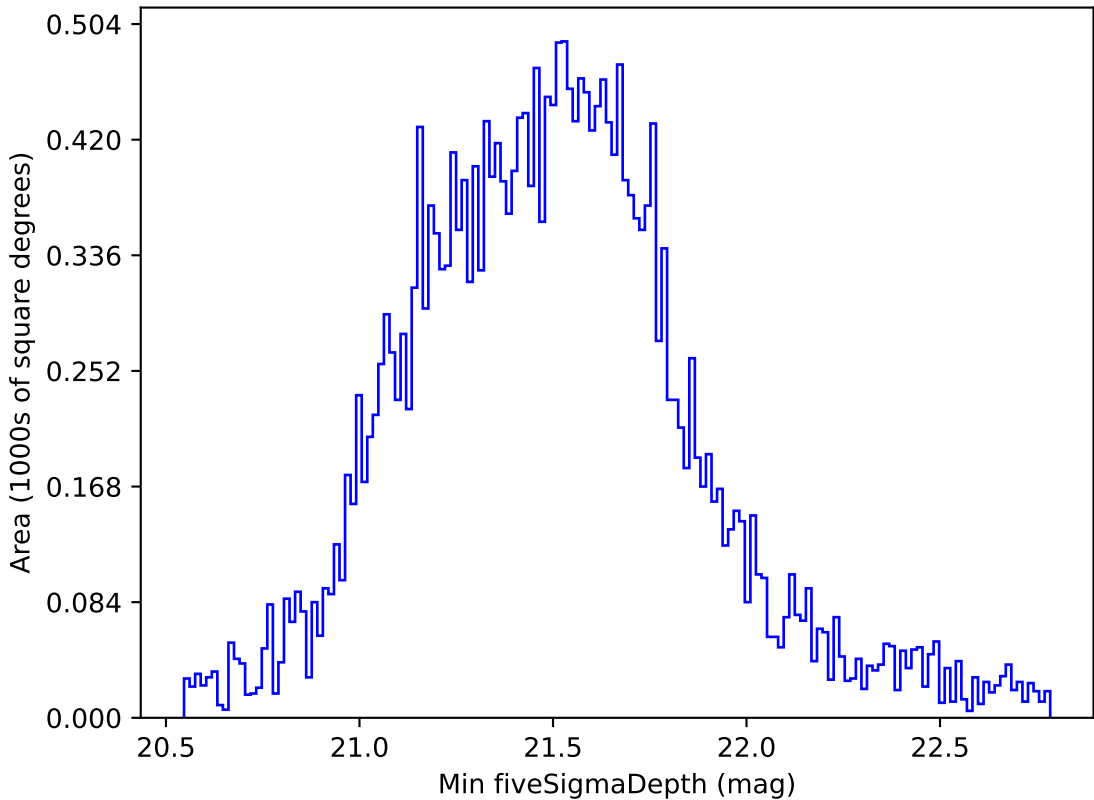
weather_cloudso0v3.5_10yrs Yr 1 all bands: Min fiveSigmaDepth
