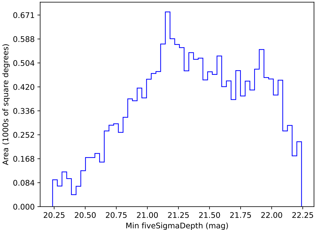
weather_cloudso0v3.5_10yrs WFD z band: Min fiveSigmaDepth
