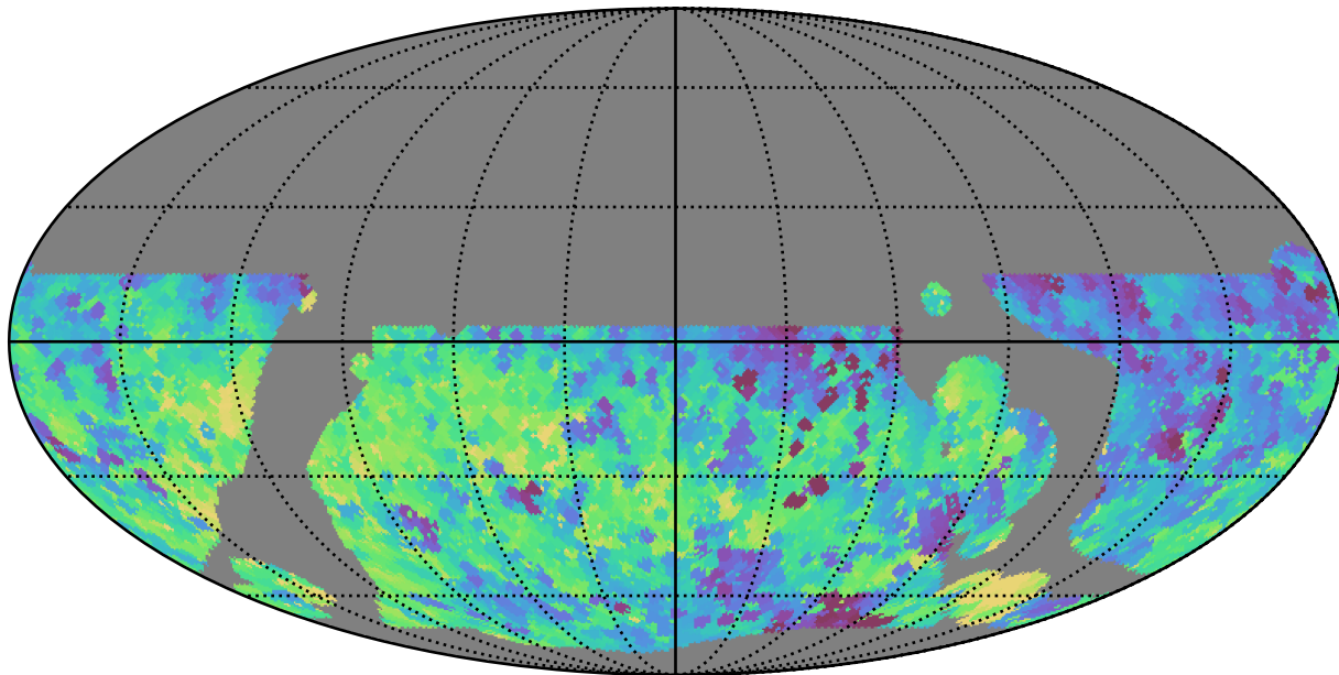
weather_cloudso0v3.5_10yrs WFD y band: Min fiveSigmaDepth
