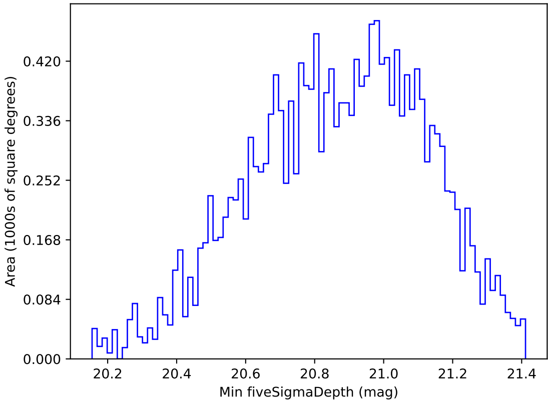
weather_cloudso0v3.5_10yrs WFD y band: Min fiveSigmaDepth
