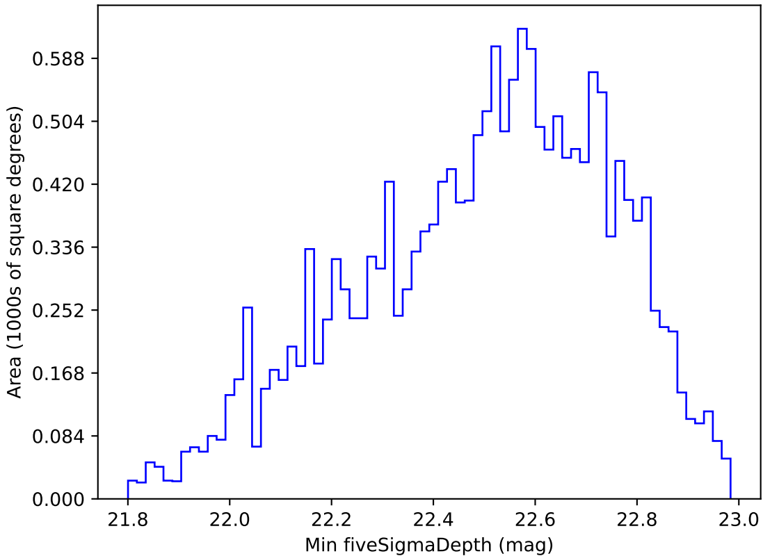
weather_cloudso0v3.5_10yrs WFD u band: Min fiveSigmaDepth
