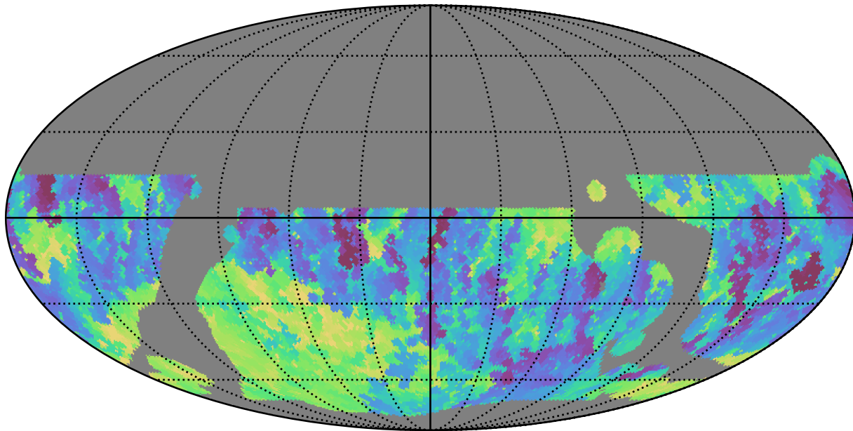
weather_cloudso0v3.5_10yrs WFD r band: Min fiveSigmaDepth
