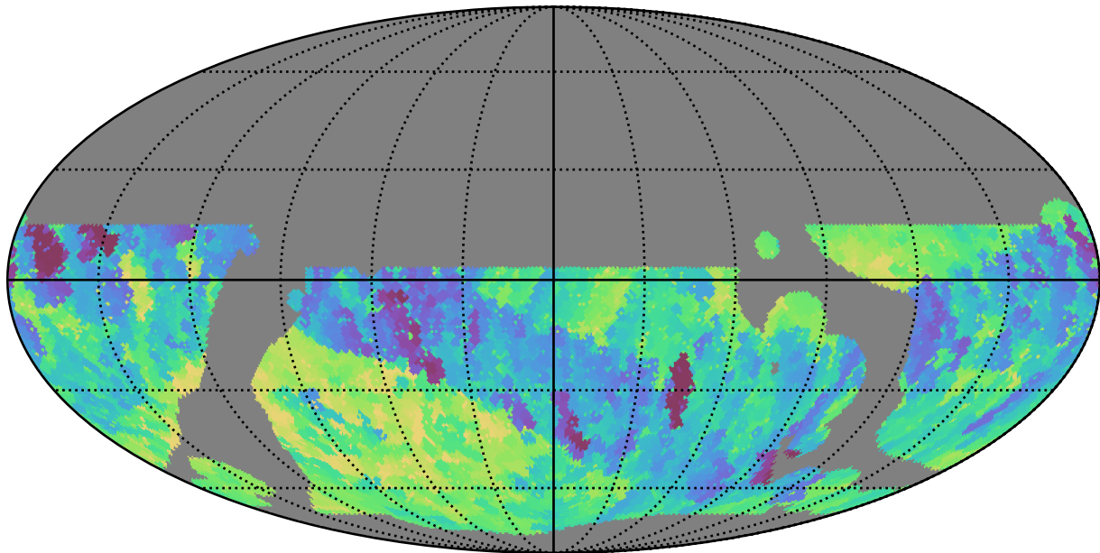
weather_cloudso0v3.5_10yrs WFD i band: Min fiveSigmaDepth
